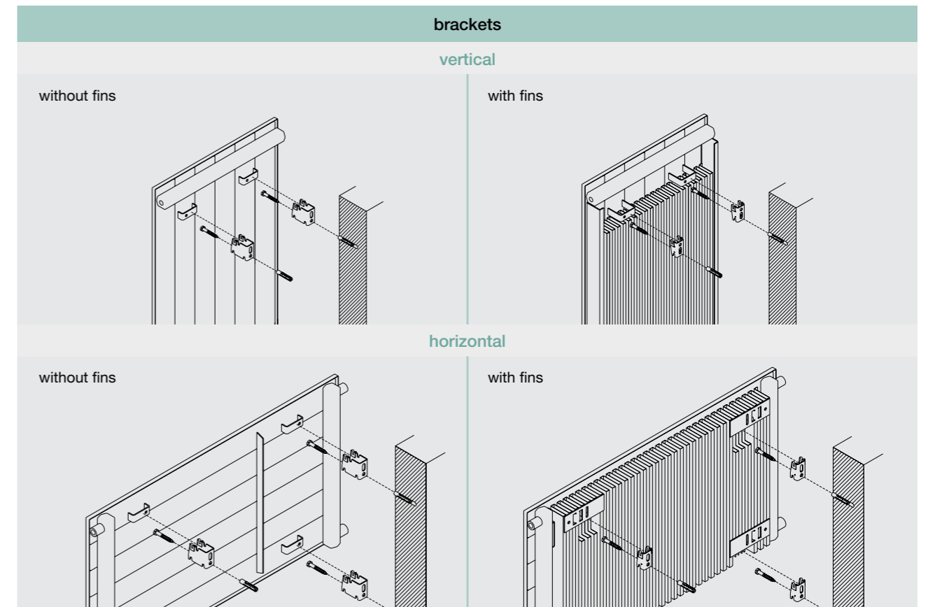
projection from wall to front face: 74mm
